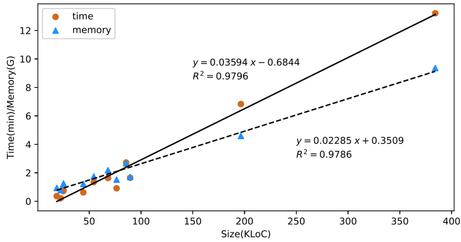
Fig. 8. Time and memory overheads of CRES.
